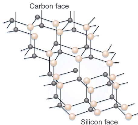
Figure 2.3: A 4H-SiC three-dimensional lattice structure [13].
