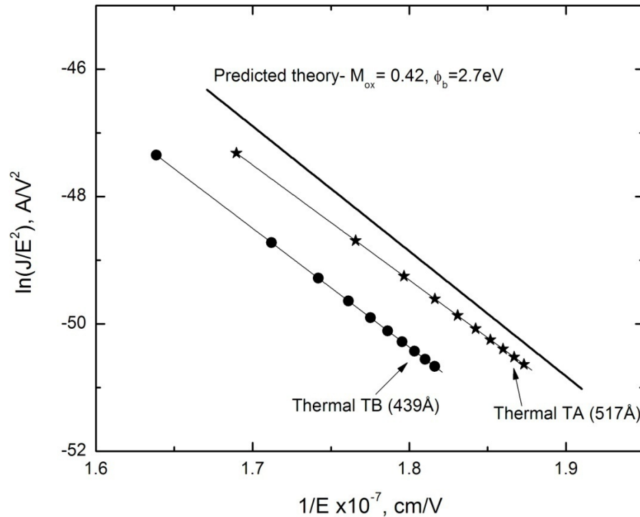
Figure 4.8: Fowler-Nordheim plot of thermal annealed oxides.
