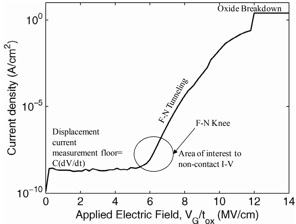
Figure 4.14: Example of current-voltage characteristics of a 4H-SiC MOS capacitor with a 500 Å gate oxide measured at room temperature [52].
